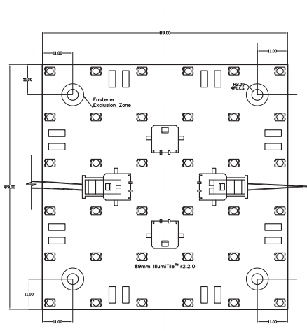
IllumiTile Top View
